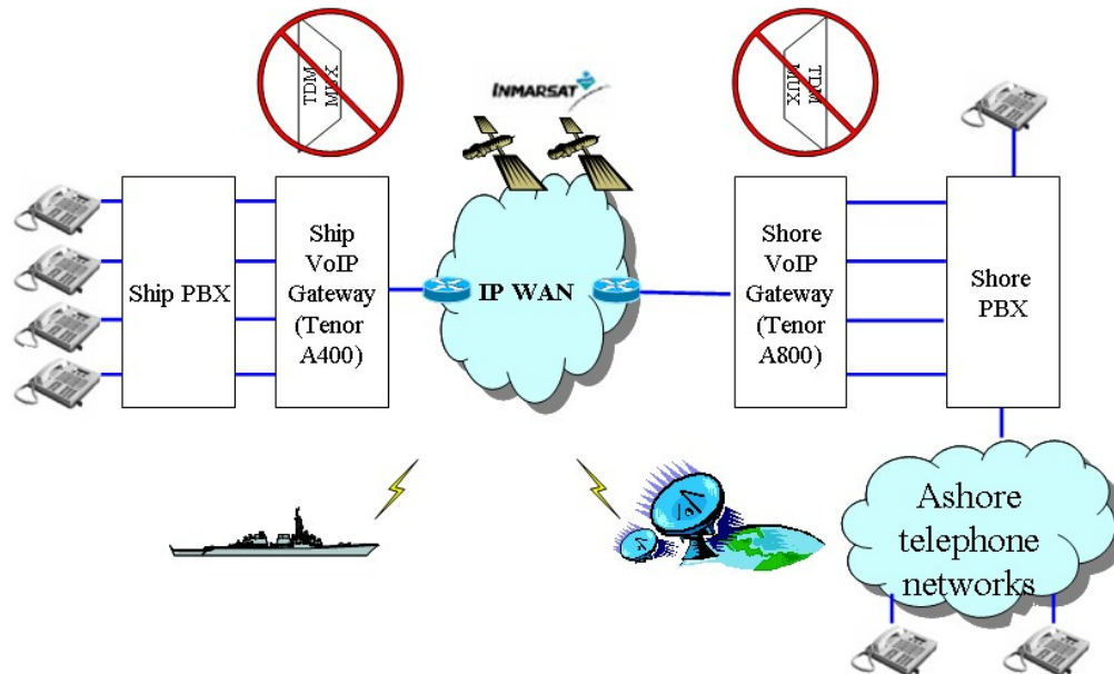
Ship-to-shore VoIP trunking across low-bandwidth satellite links
